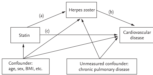
Supplementary Figure 1. The association of statin, herpes zoster, and cardiovascular disease with measured and unmeasured confounding variables. BMI, body mass index.
